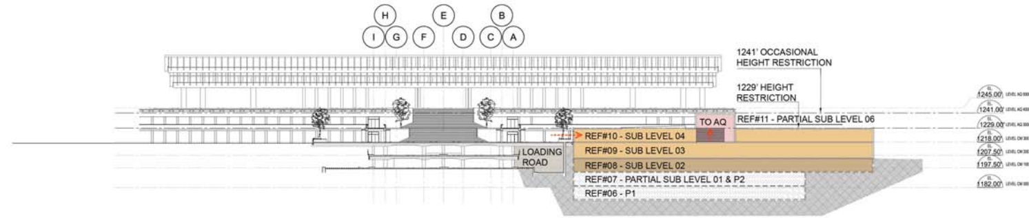
NORTH/SOUTH SITE SECTION: BUILDING LEVELS
